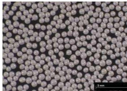
Picture 4: Microscope picture of Zirshot®-Y; round shape, smooth surface, tight size distribution
