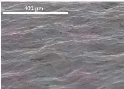
Picture 2: SEM picture of the surface condition after 2 nd step peening with Zirshot®. The surface has been smoothed; no more visible surface defect
