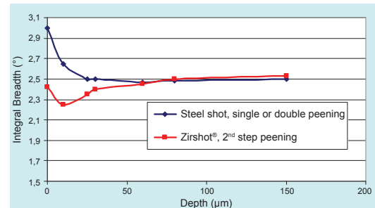
Chart 5: Dislocation density (integral breadth of diffraction pick) is much lower after peening with Zirshot® vs. steel shot
