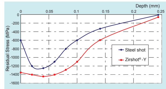
Chart 3: With comparable depth of compressive layer, residual stress profiles show much higher compressive stress at the surface after peening with Zirshot®-Y ceramic shot vs. Steel shot
